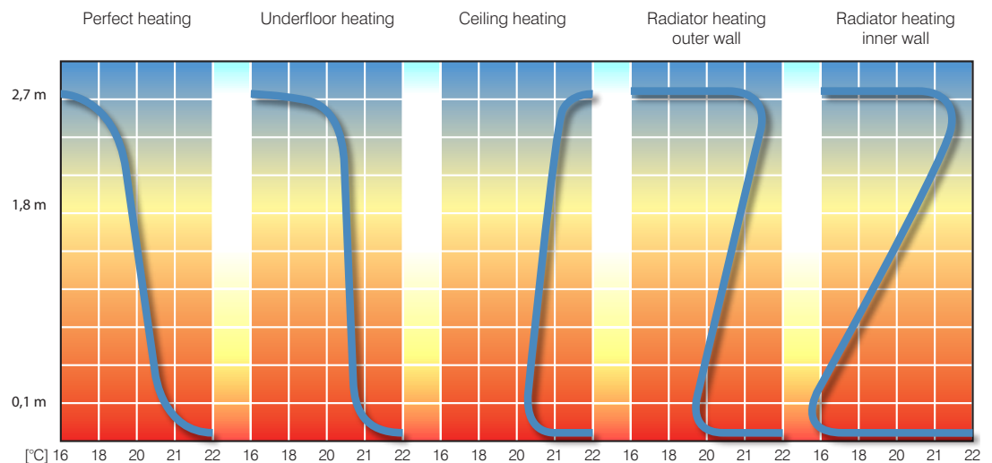
Vertical distribution of temperature for various types of heating
