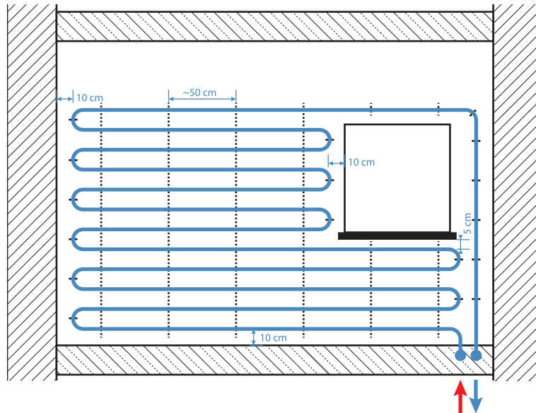
Mounting distances in wall heating
